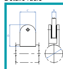
Detalle radio
