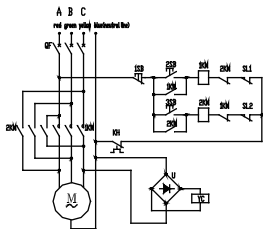
Tianyi Series 380V Electric Wiring Diagram
