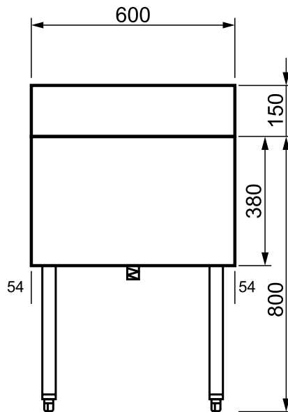
Vista Frontal
