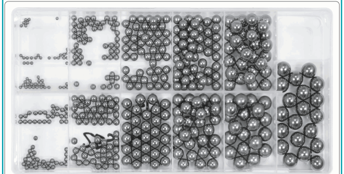
50x 3/32" (2.4 mm), 50x 1/8" (3.2 mm), 50x 5/32" (4.0 mm), 50x 3/16" (4.8 mm), 50x 7/32" (5.6 mm), 50x 1/4" (6.3 mm), 50x 9/32" (7.1 mm), 30x 5/16" (7.9 mm), 50x 11/32" (8.7 mm), 20x 3/8" (9.5 mm), 20x 13/32" (10.3 mm)
